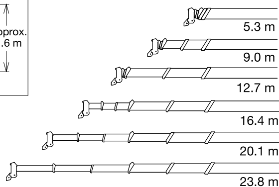
Boom Length
